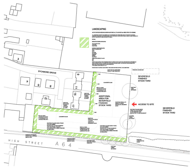
PROPOSED SITE PLAN 1:500
