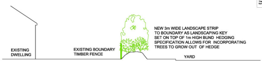
PROPOSED SECTION TO BOUNDARY TO SYCAMORE CLOSE 1:100
